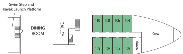
Main Deck
